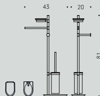
B9903 Piantana (Base 24x14 cm) con porta salvietta, porta sapone, porta rotolo e porta scopino sospeso in vetro acidato Floor standing column with towel holder, soap holder, paper holder and suspended acid glass brush holder
