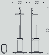
B9816 Piantana (Base 22 cm) con porta rotolo e porta scopino sospeso in vetro acidato Floor standing column with paper holder and suspended acid glass brush holder
